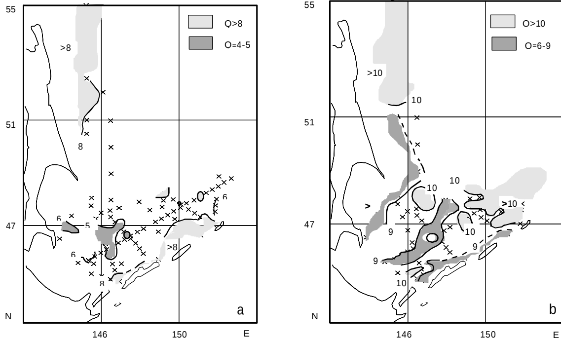
Fig. 5 Isopycnal potential vorticity (f/r)(\partial r/\partial z)(10^{-11} \text{ m}^{-1} \text{ s}^{-1}) at (a) 26.85 s_q and (b) 27.05 s_q .
