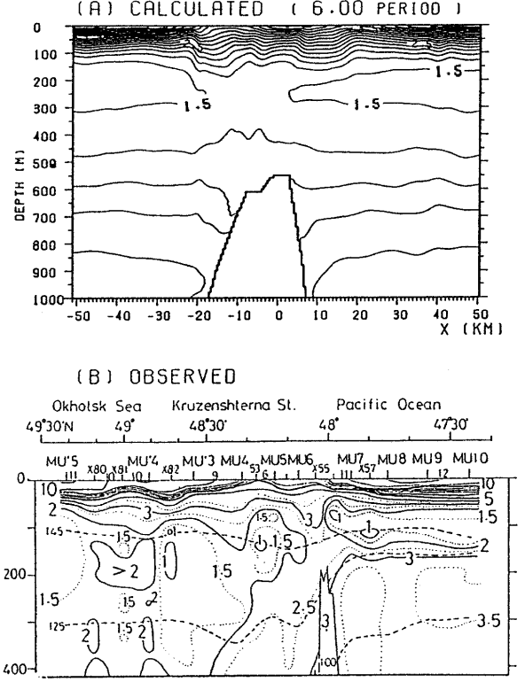
Fig. 5 (a) The calculated potential temperature distribution after 6 periods, and (b) the observed potential temperature distribution in the Kruzenshterna Strait.
