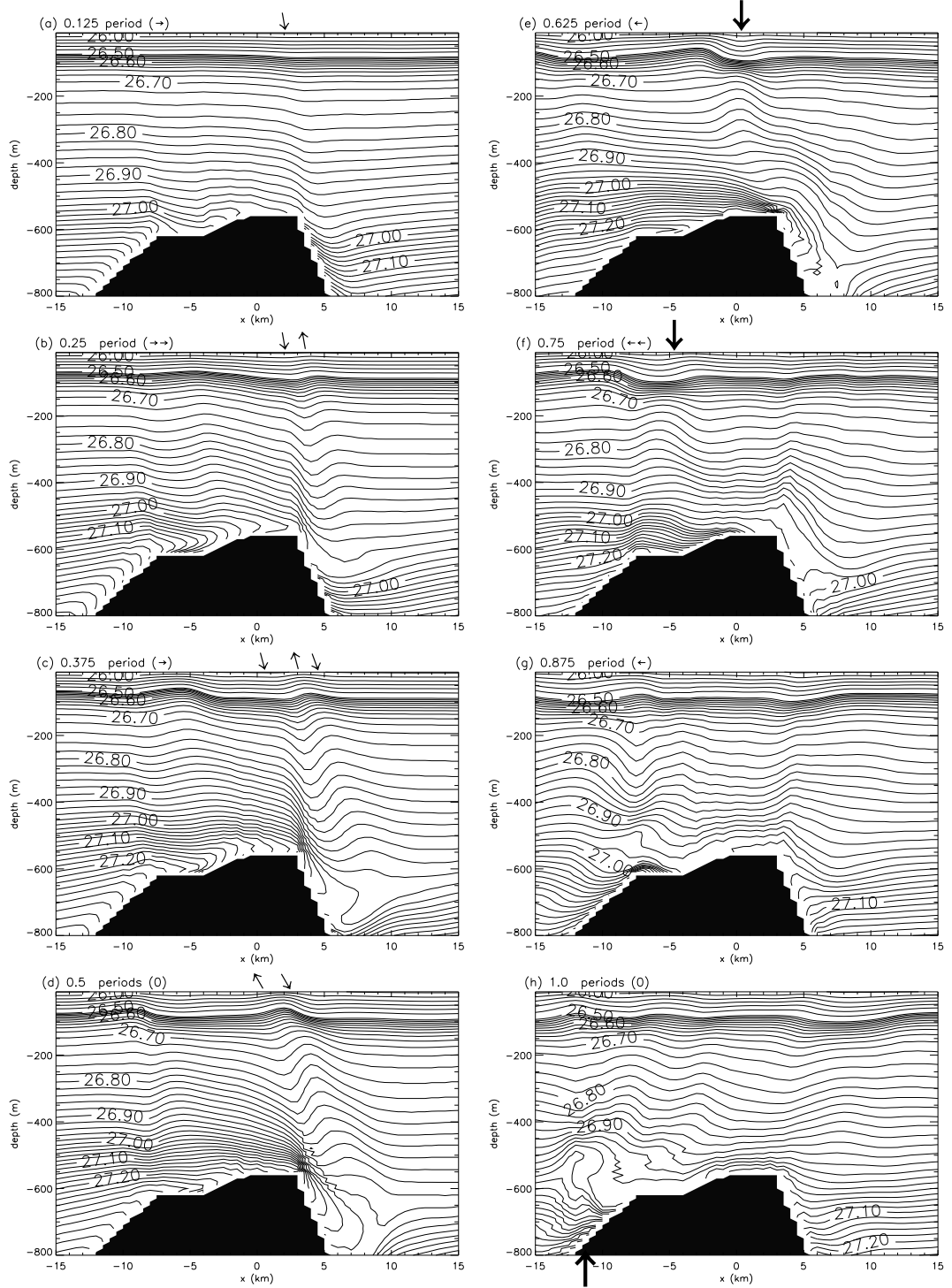
Fig. 4 The evolution of potential density ( \sigma_\theta ) around the sill top in the K_1 case, during the first period, after (a) 0.125, (b) 0.25, (c) 0.375, (d) 0.5, (e) 0.625, (f) 0.75, (g) 0.875, (h) 1 period, when the generation process of the large-amplitude unsteady lee wave can be clearly seen. For \sigma_\theta < 26.5 , the contour interval is 0.1 \sigma_\theta . For \sigma_\theta \geq 26.5 the contour interval is 0.02 \sigma_\theta .
