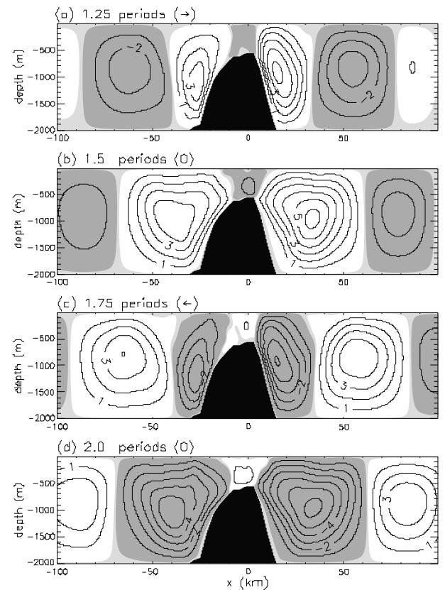
Fig. 2 The time series of the internal mode stream function in the M_2 case during the second tidal period; after (a) 1.25, (b) 1.5, (c) 1.75, and (d) 2.0 periods. The contour interval is 1.0 \times 10^5 \text{ cm}^2 \text{ s}^{-1} . Values in unshaded areas and the darkly shaded areas are positive and negative, respectively, and the absolute values in the lightly shaded areas are less than 1 \times 10^4 \text{ cm}^2 \text{ s}^{-1} .
