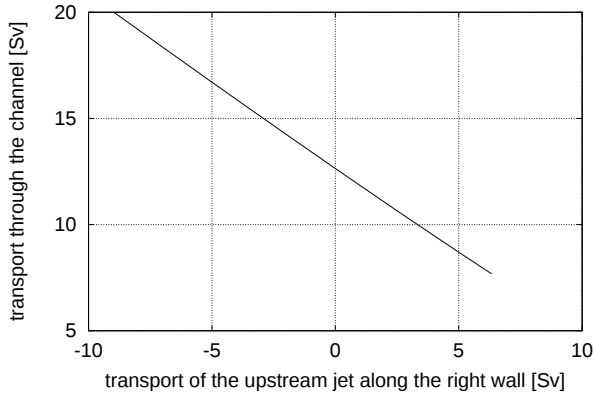
Fig. 6 Transport through the strait as a function of the transport of the upstream jet along the right side of the coast. The estimation is based on Gill's hydraulic model (1977) of constant potential vorticity flow. See the text for details.
