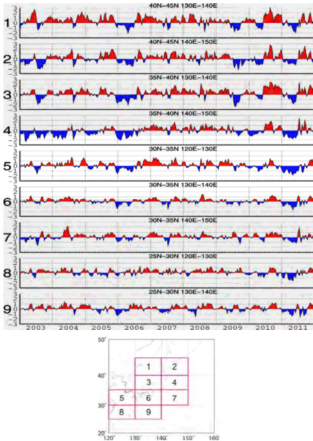
Fig. 2 Time series of 10-day mean SST anomalies ( ^{\circ}\text{C} ) averaged for the sub-areas shown in the bottom panel. Anomalies are deviations from JMA's 1971–2000 climatology.
