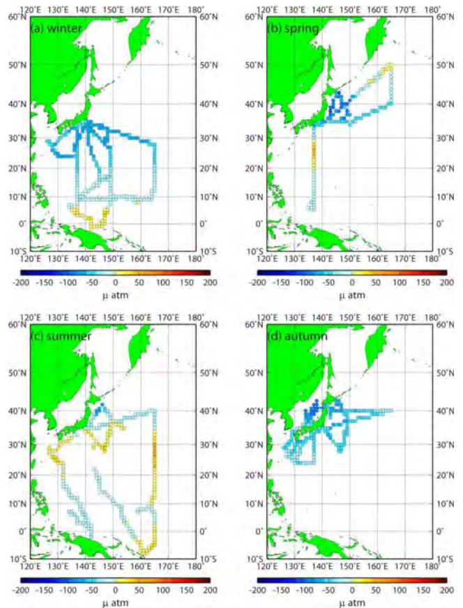
Fig. 4 Difference in \text{CO}_2 partial pressure between the ocean and the atmosphere in the western North Pacific in 2011: (a) winter (January–March), (b) spring (April–June), (c) summer (July–September) and (d) autumn (October–December).
